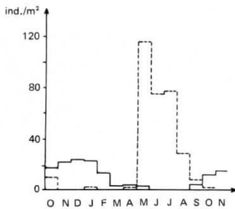
Fig. 6: Monthly average density of Macrargus rufus . Solid line: adults; dashed line: juveniles.
