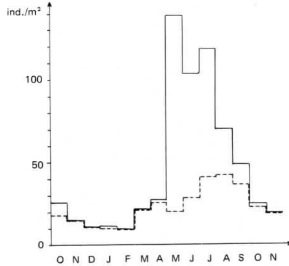
Fig. 3: Monthly average density of juveniles. Solid line: with Macrargus rufus ; dashed line: without M. rufus .
