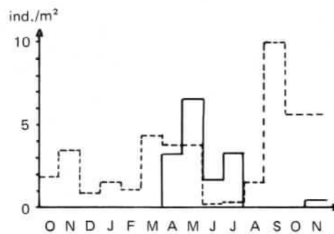
Fig. 8: Monthly average density of Diplocephalus picinus . Solid line: adults; dashed line: juveniles.
