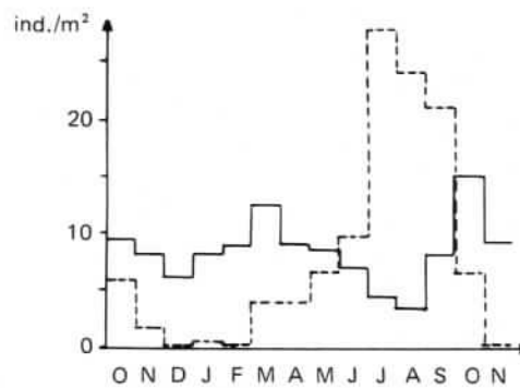
Fig. 7: Monthly average density of Microneta viaria . Solid line: adults; dashed line: juveniles.
